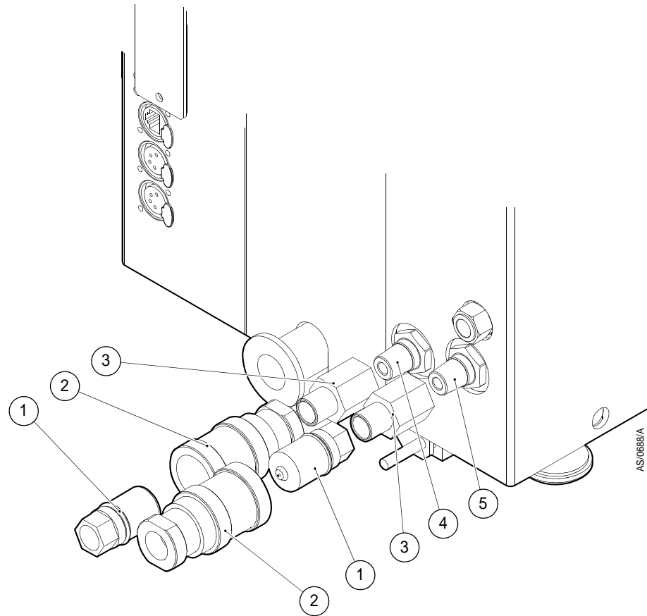
Figure 10 - Installing 3/8" quick connect fittings (provided)
